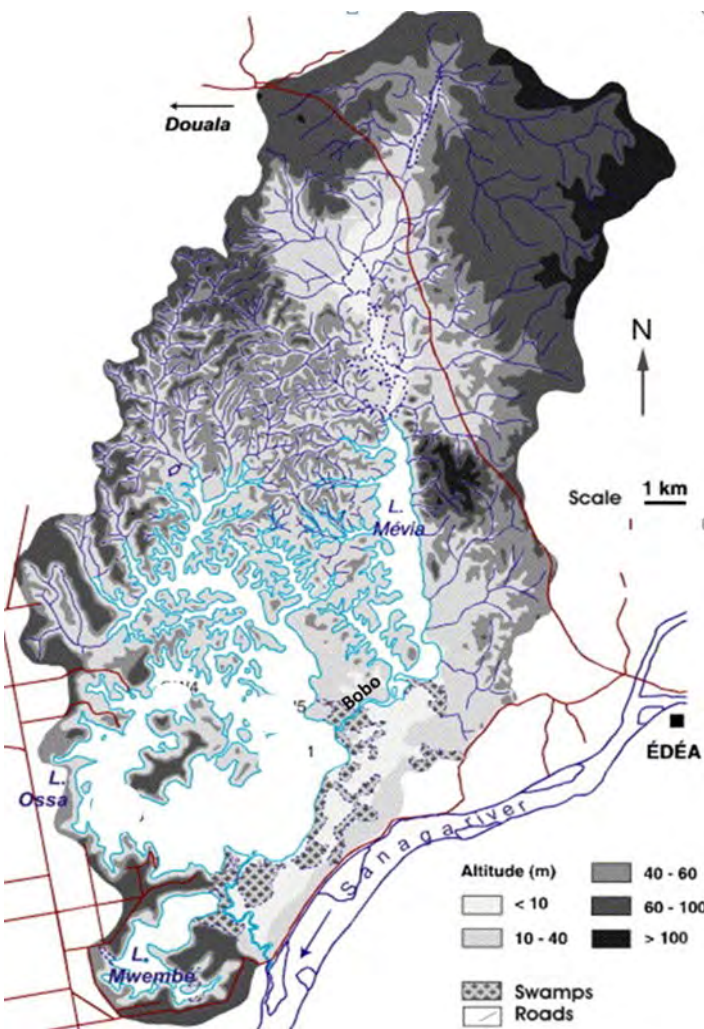
Figure 1: Topographic map of the The Lake Ossa complex showing the three lakes (modified from Giresse, 2005)
