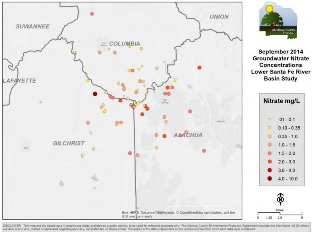
Figure 2a. Groundwater Nitrate Results Map, September 2014
