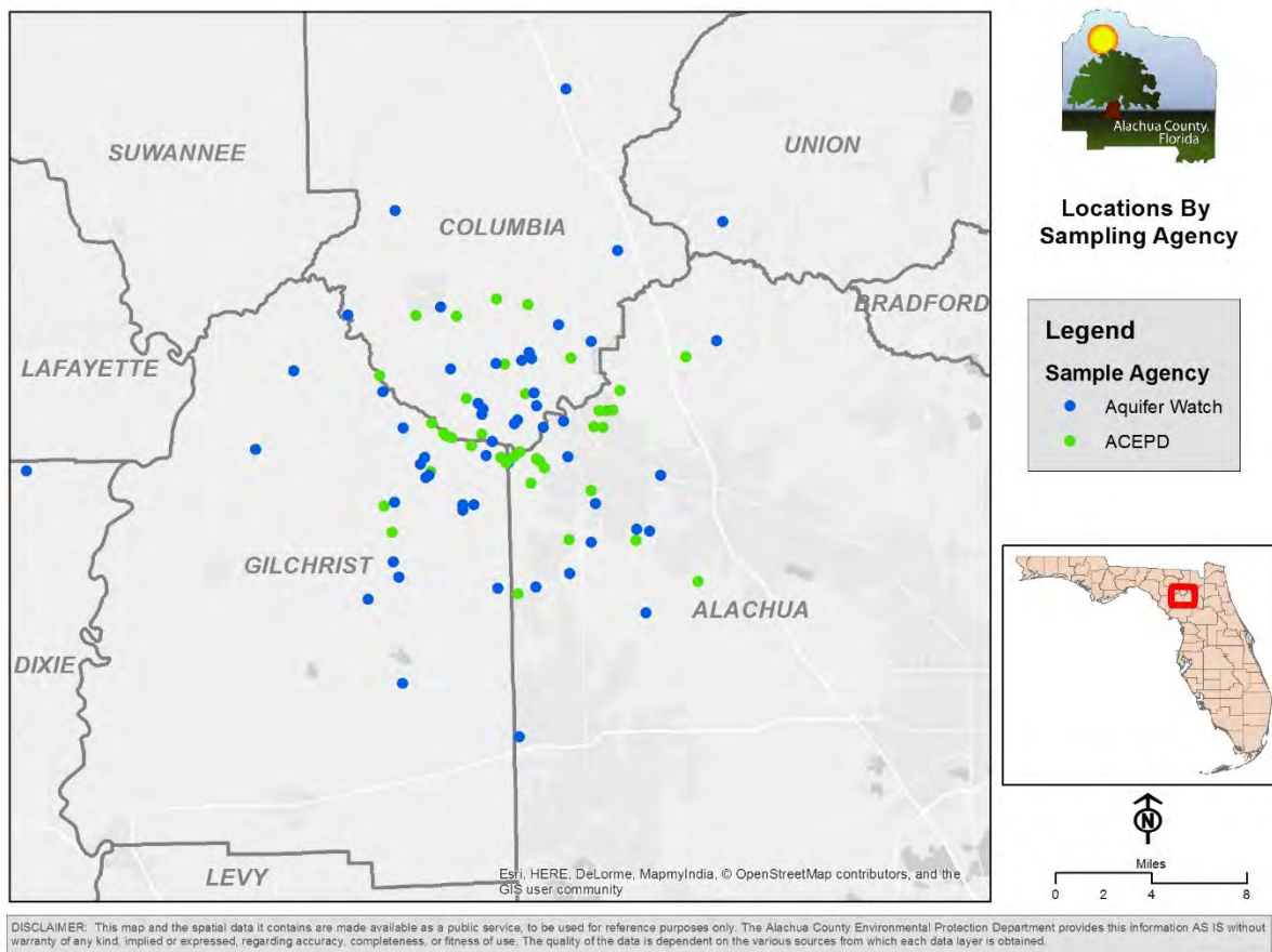
Figure 1. Sample locations in Lower Santa Fee River Basin. Samples obtained in September 2014 and May 2015.
