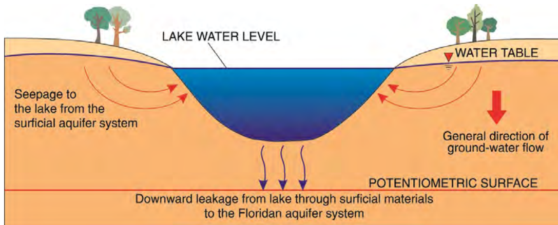
Groundwater seepage
