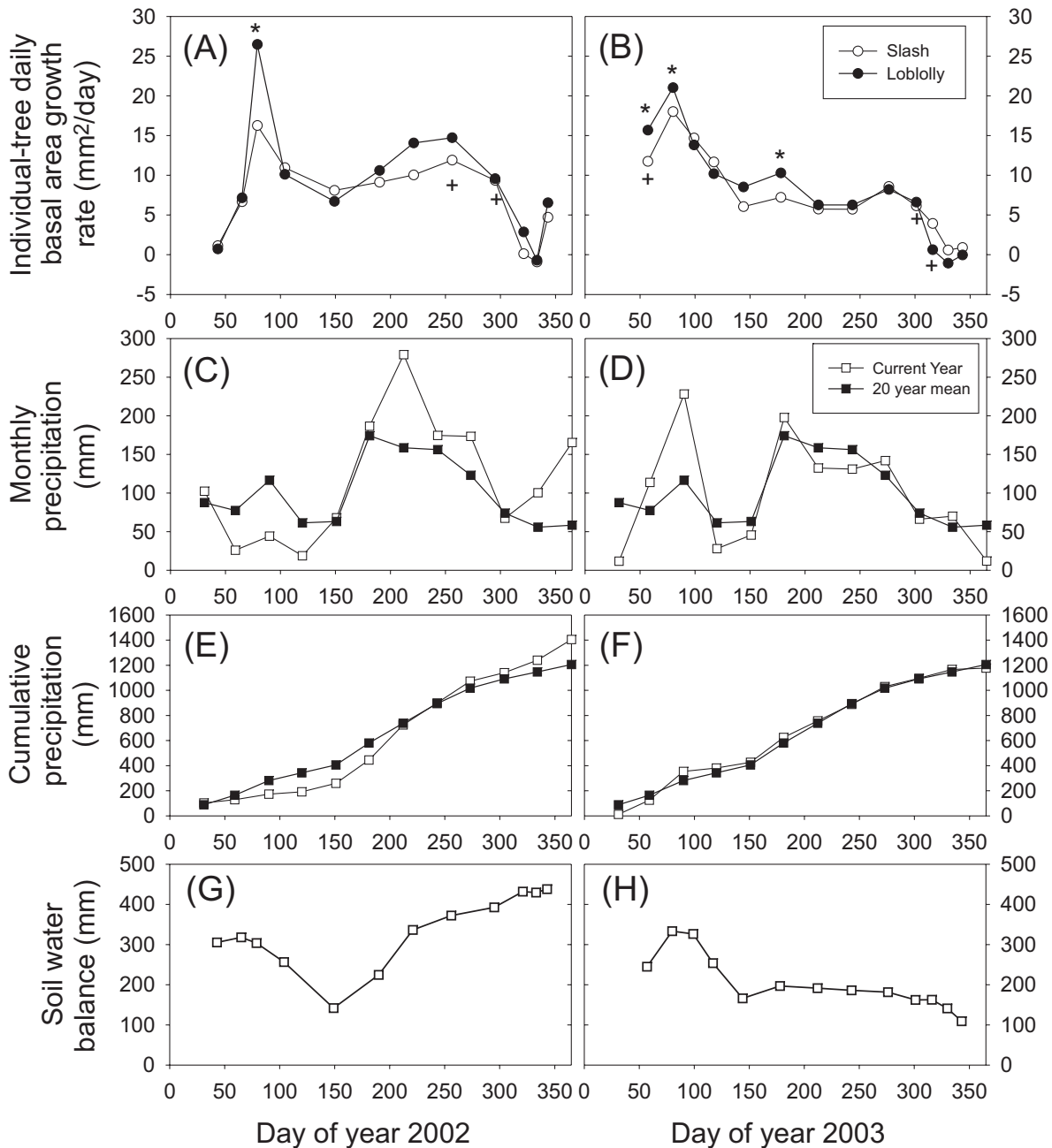
Fig. 2. Species mean daily basal area growth increment in 2002 (A) and 2003 (B) for loblolly and slash pines in north-central Florida, where an asterisk indicates significant differences between species ( P < 0.05 ) and a plus indicates significant differences among slash pine families ( P < 0.05 ); current-year and 20-year mean monthly precipitation in 2002 (C) and 2003 (D); cumulative precipitation in 2002 (E) and 2003 (F); and mean plot-level soil water balance (error bars indicating standard error) in 2002 (G) and 2003 (H). Precipitation data from Gainesville Regional Airport, NOAA (2003).
