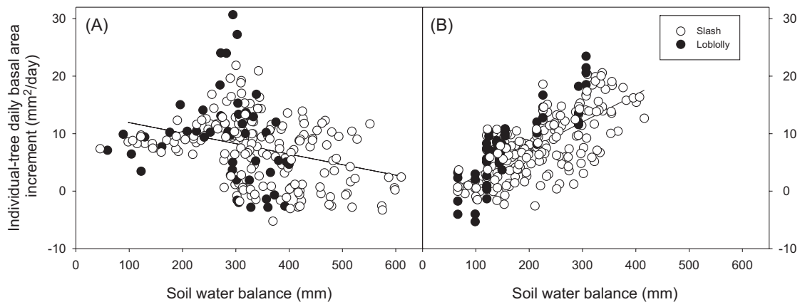
Fig. 3. Relationship between individual-tree daily basal area (BA) increment and simulated daily plot-level soil water balance in loblolly and slash pines in 2002 (A) and 2003 (B). The line shows a linear regression through data. (A) Daily BA growth = 13.7929 - 0.0187 \times (\text{soil water balance}) ; R^2 = 0.11 , P < 0.0001 . (B) Daily BA growth = -1.9424 + 0.0478 \times (\text{soil water balance}) ; R^2 = 0.49 , P < 0.0001 .
